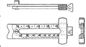
Fig 12. Planche mobile.
